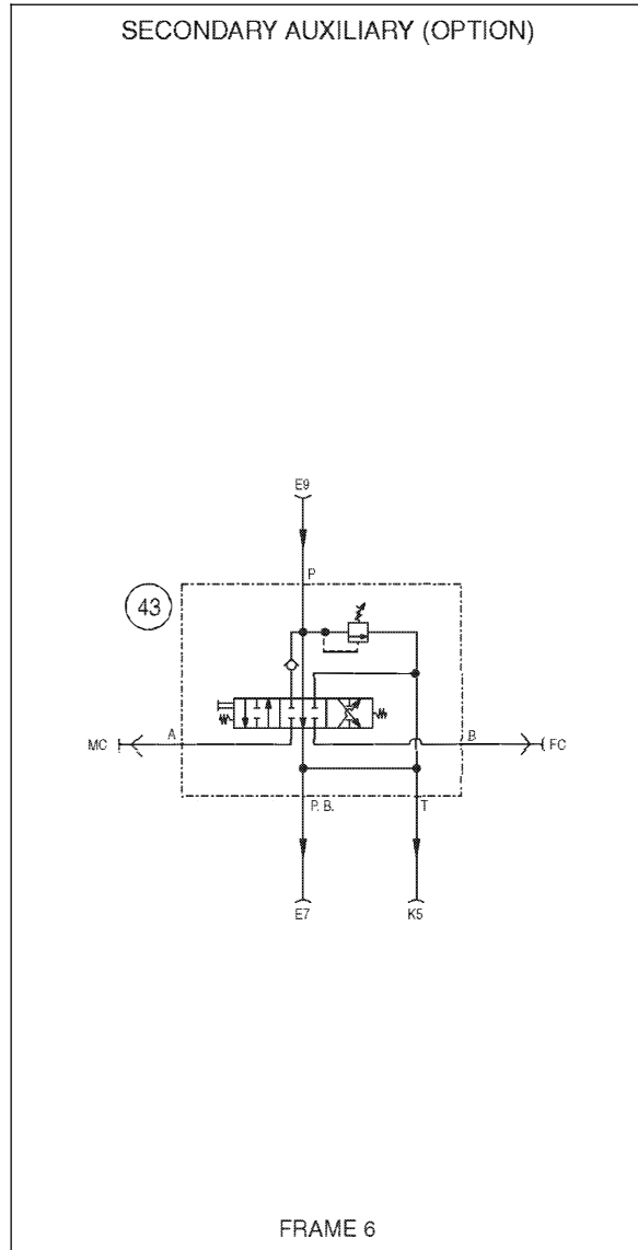
43. Secondary auxiliary control valve
