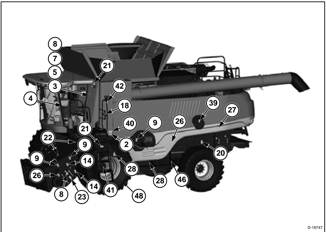
FIG. 47 FIG. 47: Front, Left-hand View.
